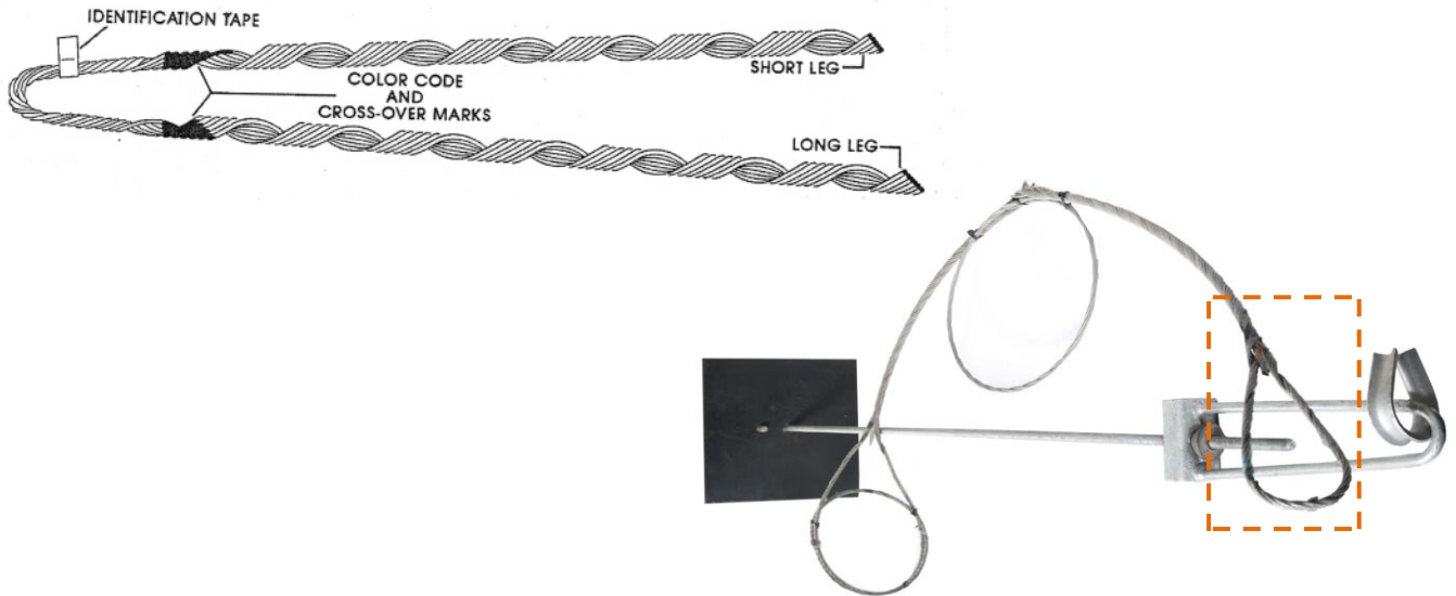
Stay set with base plate, adjustable rod, thimble, steel wire double wrap guy and bottom make off highlighted
